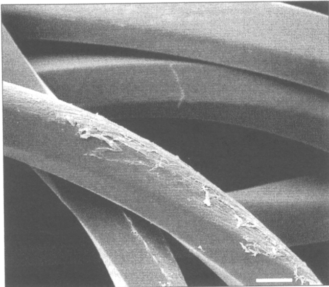
Figure 1. Photomicrograph of polyester fiber with abrasion and abrasion debris. (courtesy H.R. Bhattacharjee Ph.D. Texwipe)
