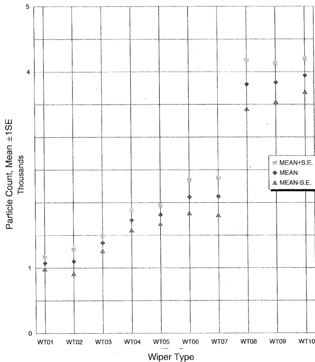
Figure 2. Graphical comparison of the abrasion rates (machine direction plus cross direction) for various types of knitted polyester.
